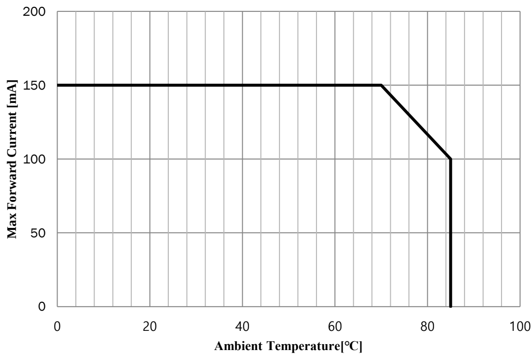
FIG 8. Max. Forward current vs Ambient Temperature (Rth J-S : 12.3°C/W)
